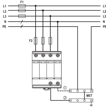
TN-S Network System, 3N
