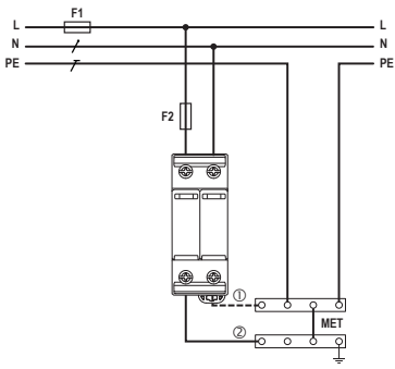
TN-S Network System, 1N
