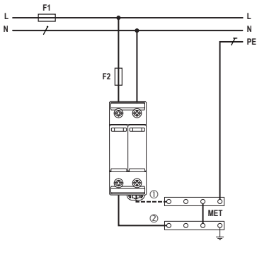
TT Network System, 1N
