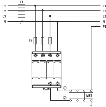
TT Network System, 3N
