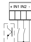
Connessione NPN NPN connection
