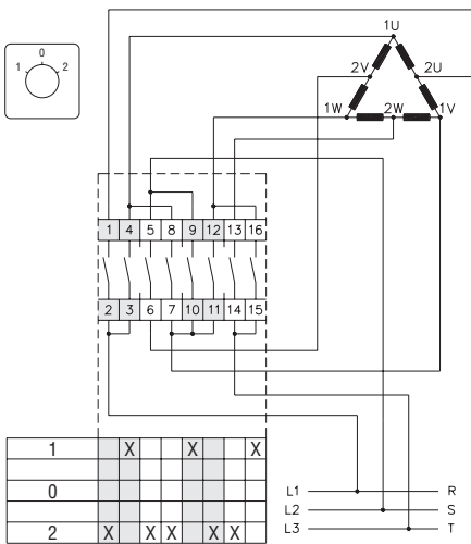
DAHLANDER MOTOR CONTROL 13
