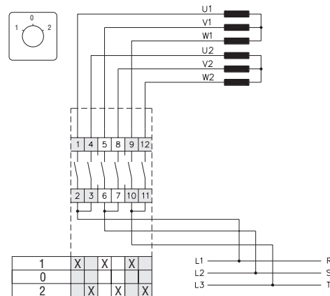
SEPARATE WINDINGS SWITCHES 53
